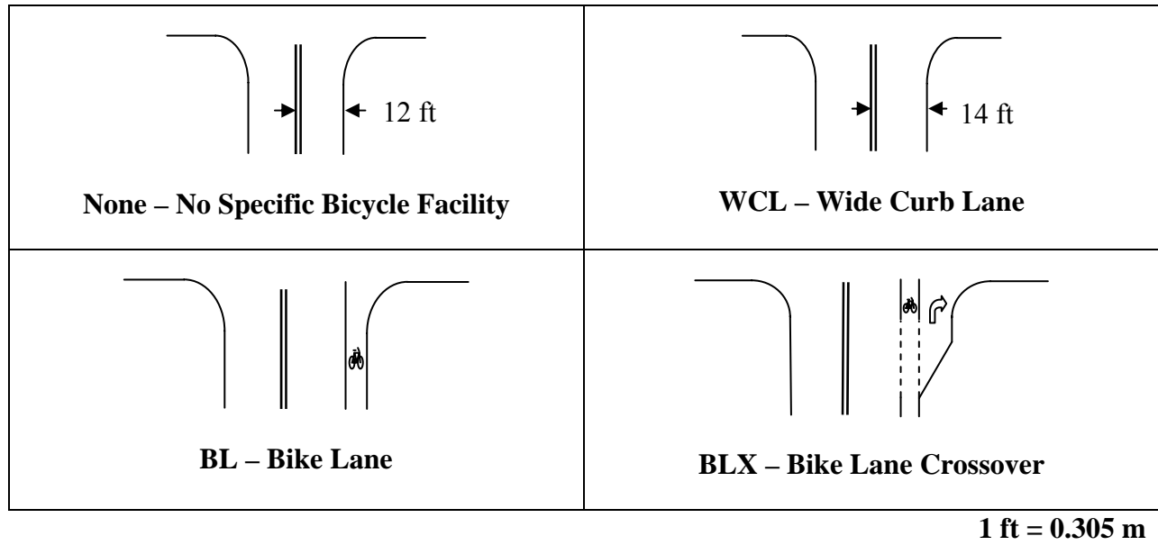
Figure 12. Bicycle facility types.
